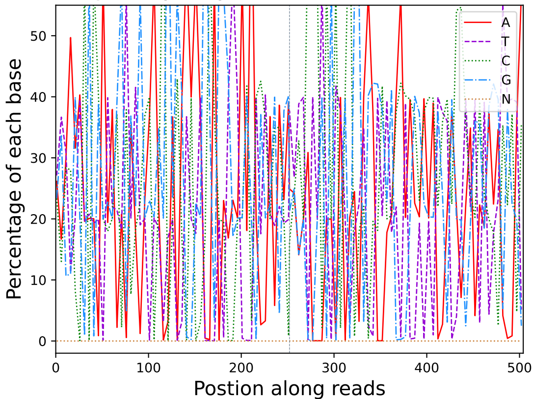
Base percentage along reads (R10415)
